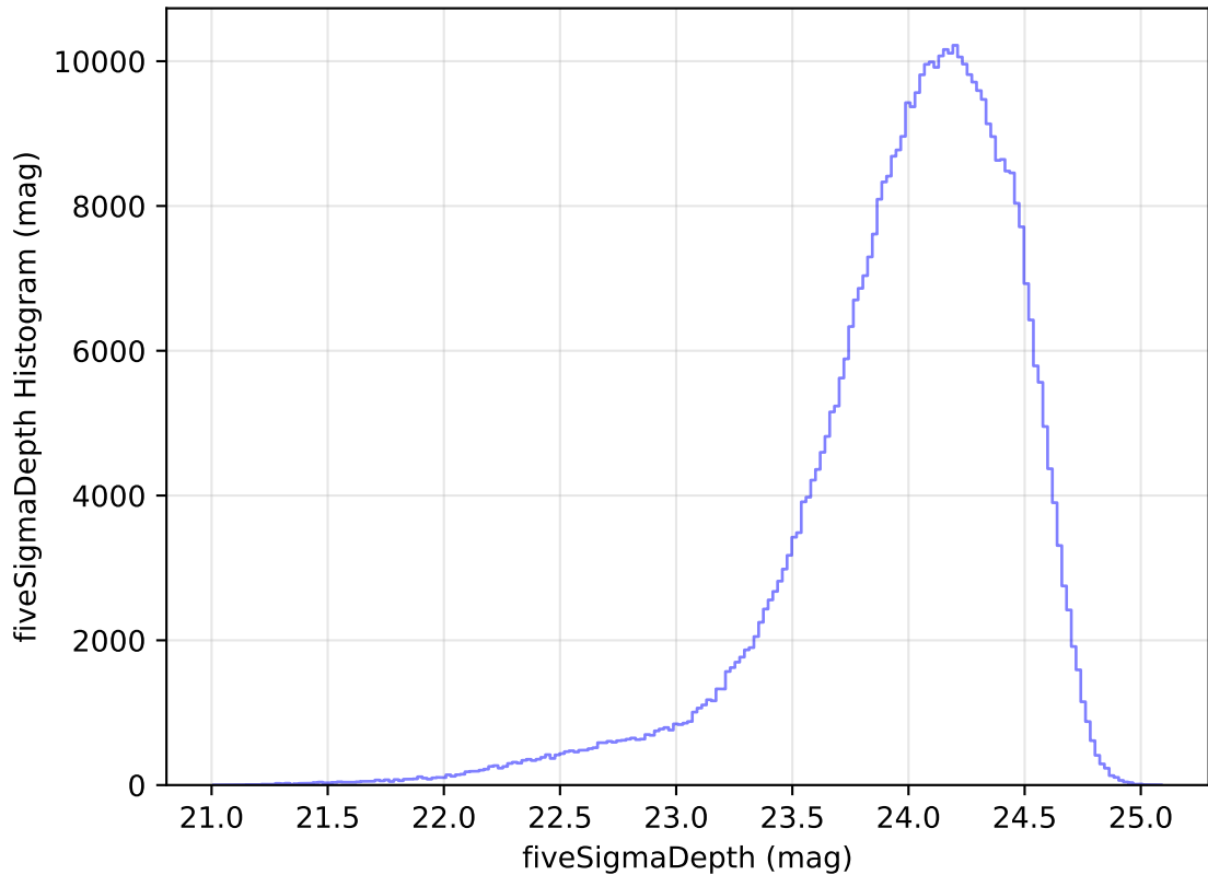
weather_cloudso2v3.4_10yrs WFD r band: fiveSigmaDepth Histogram
