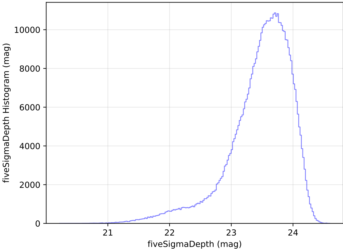
weather_cloudso2v3.4_10yrs WFD i band: fiveSigmaDepth Histogram
