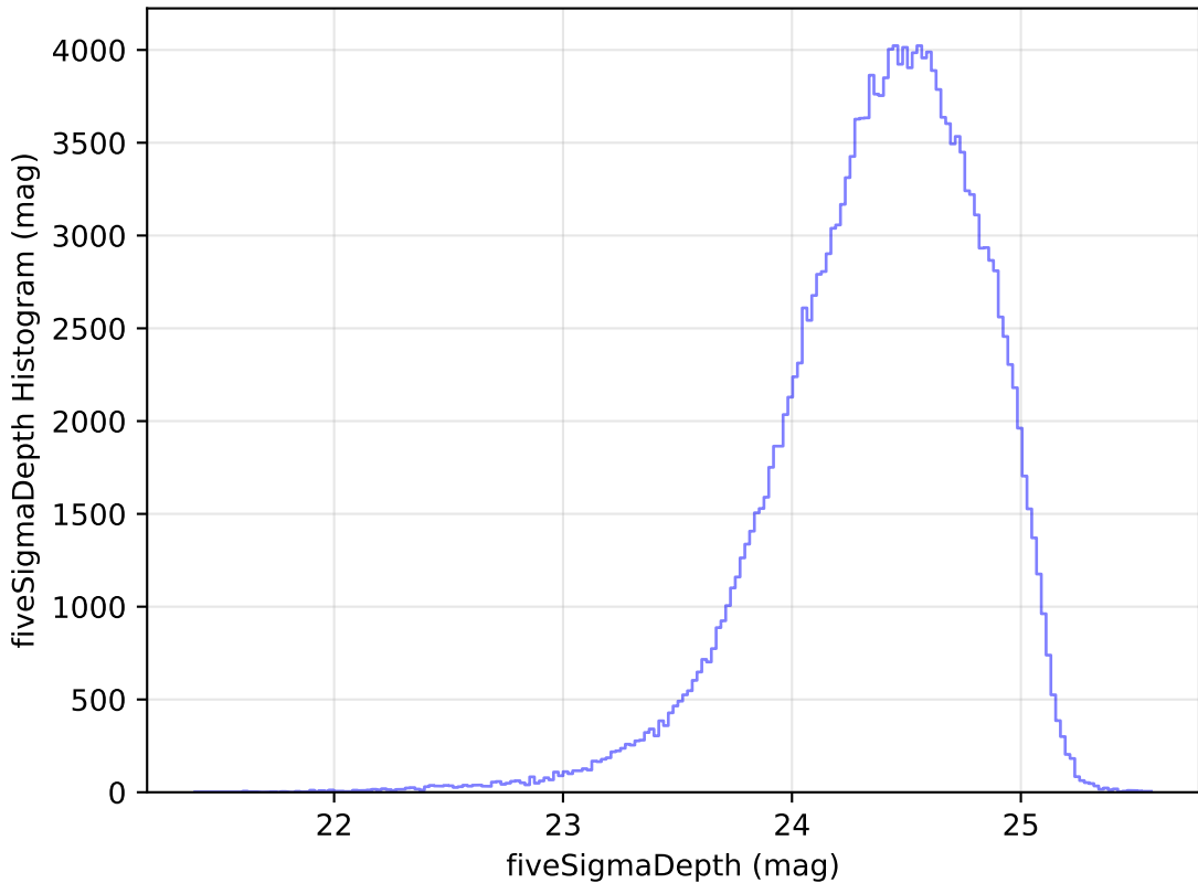
weather_cloudso2v3.4_10yrs WFD g band: fiveSigmaDepth Histogram
