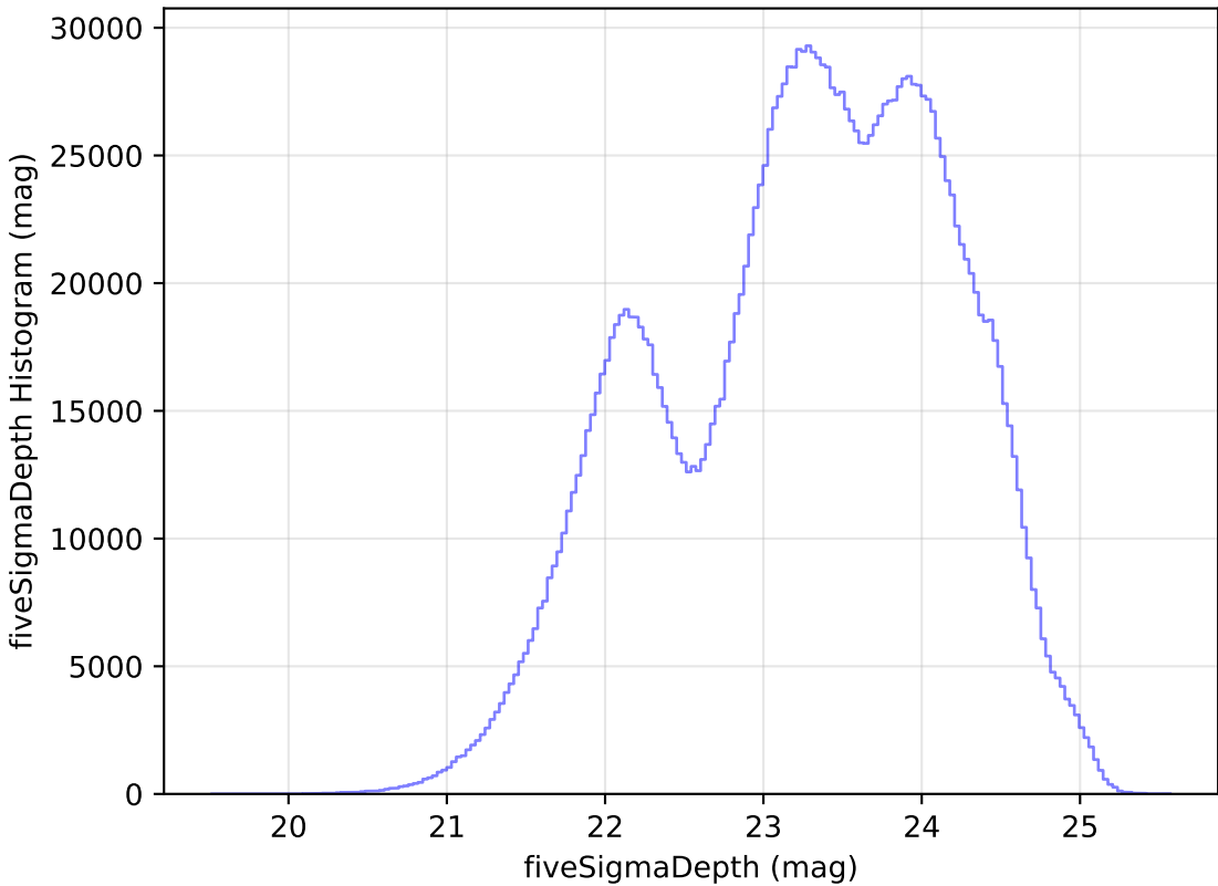
weather_cloudso2v3.4_10yrs WFD all bands: fiveSigmaDepth Histogram
