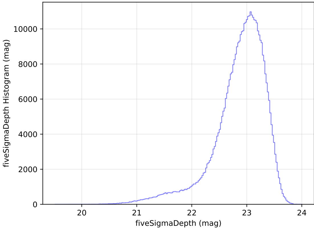
weather_cloudso2v3.4_10yrs All sky z band: fiveSigmaDepth Histogram
