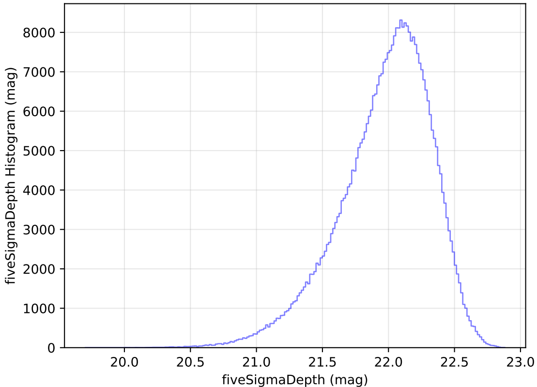
weather_cloudso2v3.4_10yrs All sky y band: fiveSigmaDepth Histogram
