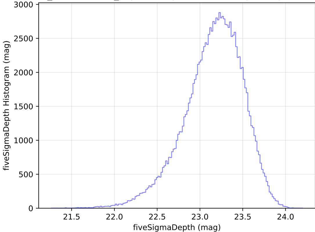
weather_cloudso2v3.4_10yrs All sky u band: fiveSigmaDepth Histogram
