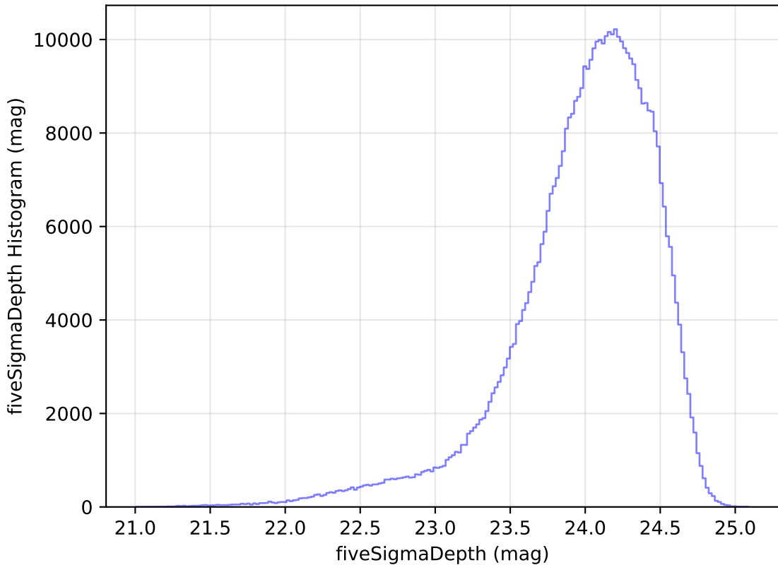
weather_cloudso2v3.4_10yrs All sky r band: fiveSigmaDepth Histogram
