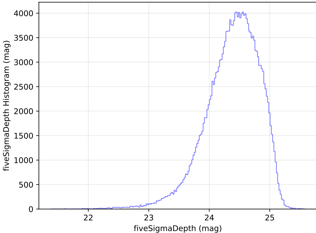
weather_cloudso2v3.4_10yrs All sky g band: fiveSigmaDepth Histogram
