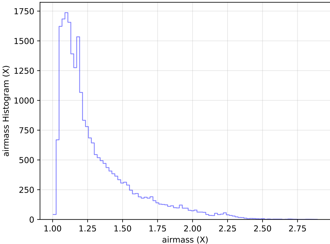
weather_cloudso2v3.4_10yrs Yr 1 g band: airmass Histogram
