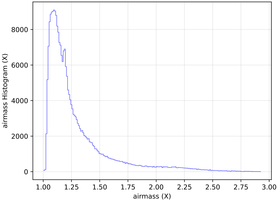
weather_cloudso2v3.4_10yrs Yr 1 all bands: airmass Histogram
