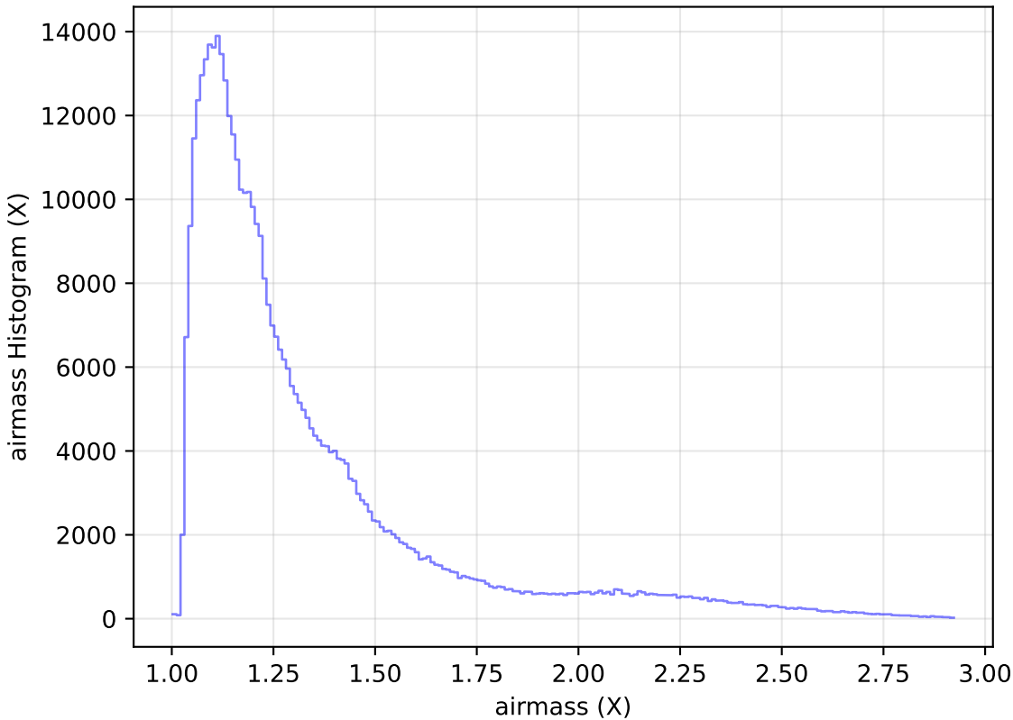
weather_cloudso2v3.4_10yrs WFD z band: airmass Histogram
