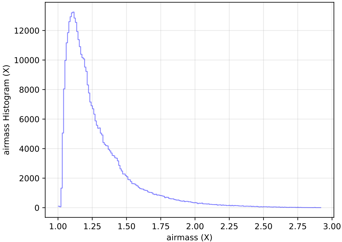
weather_cloudso2v3.4_10yrs WFD y band: airmass Histogram
