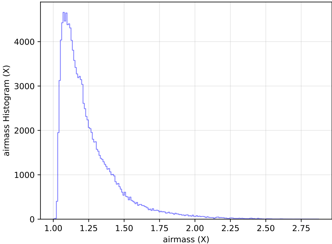
weather_cloudso2v3.4_10yrs WFD u band: airmass Histogram
