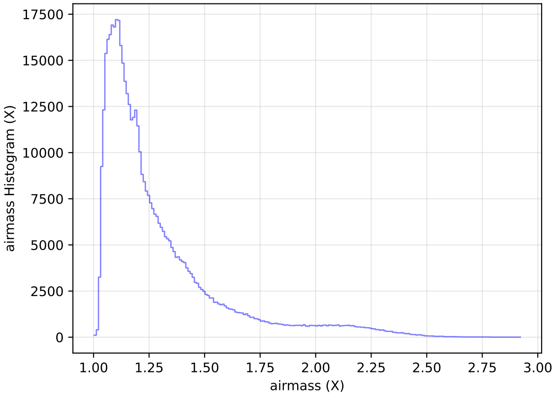
weather_cloudso2v3.4_10yrs WFD r band: airmass Histogram
