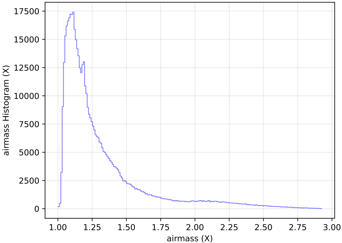
weather_cloudso2v3.4_10yrs WFD i band: airmass Histogram
