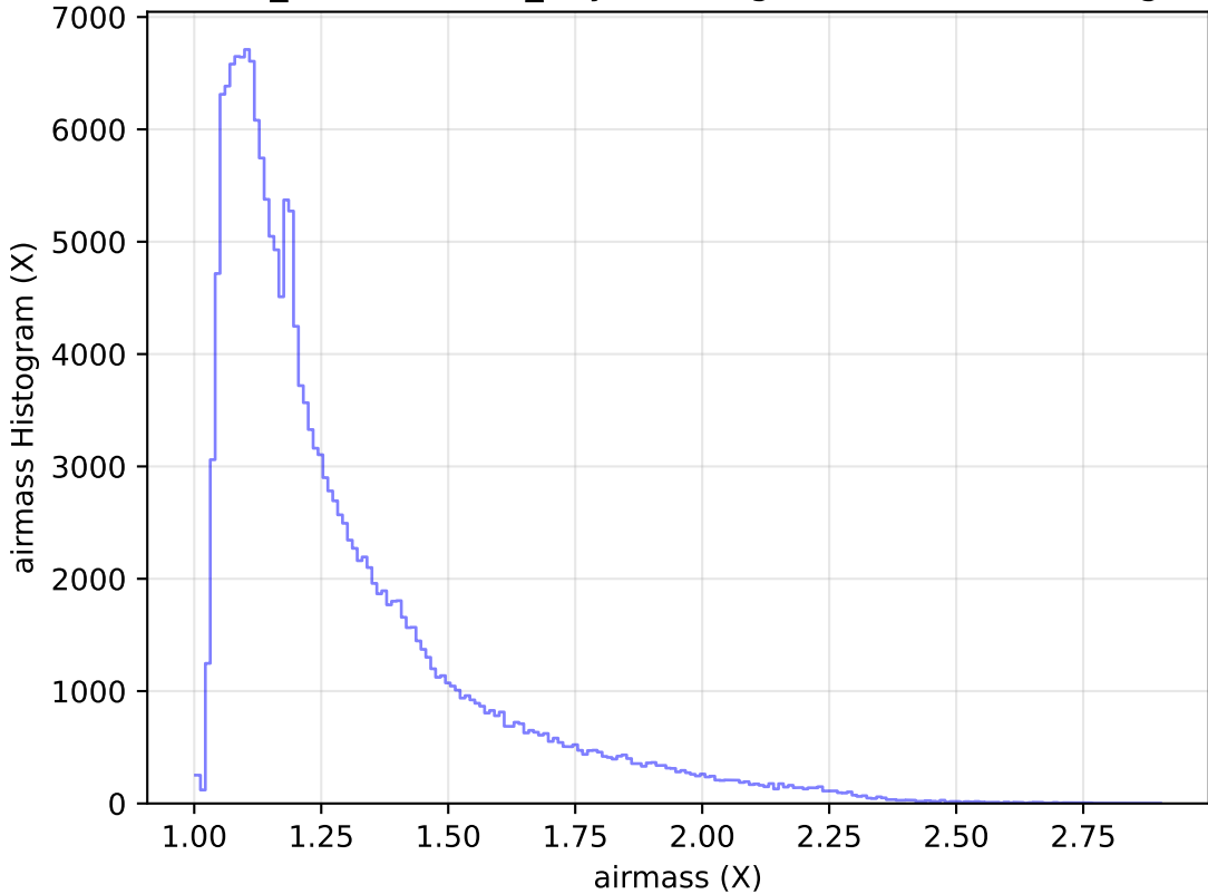
weather_cloudso2v3.4_10yrs WFD g band: airmass Histogram
