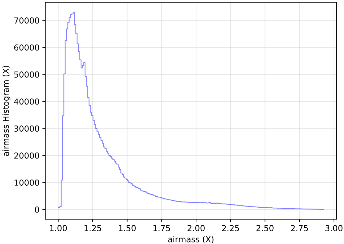
weather_cloudso2v3.4_10yrs WFD all bands: airmass Histogram
