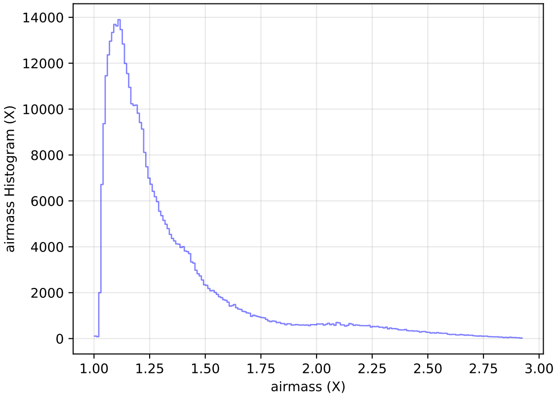
weather_cloudso2v3.4_10yrs All sky z band: airmass Histogram
