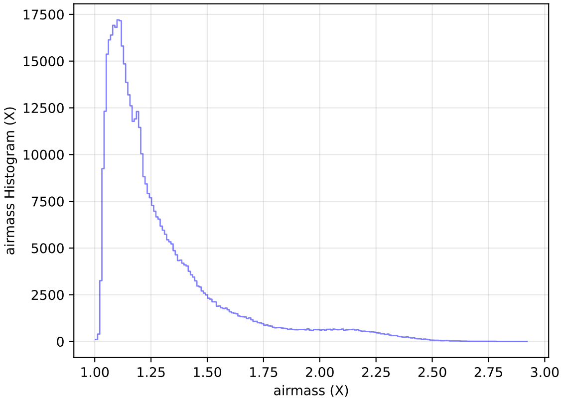
weather_cloudso2v3.4_10yrs All sky r band: airmass Histogram
