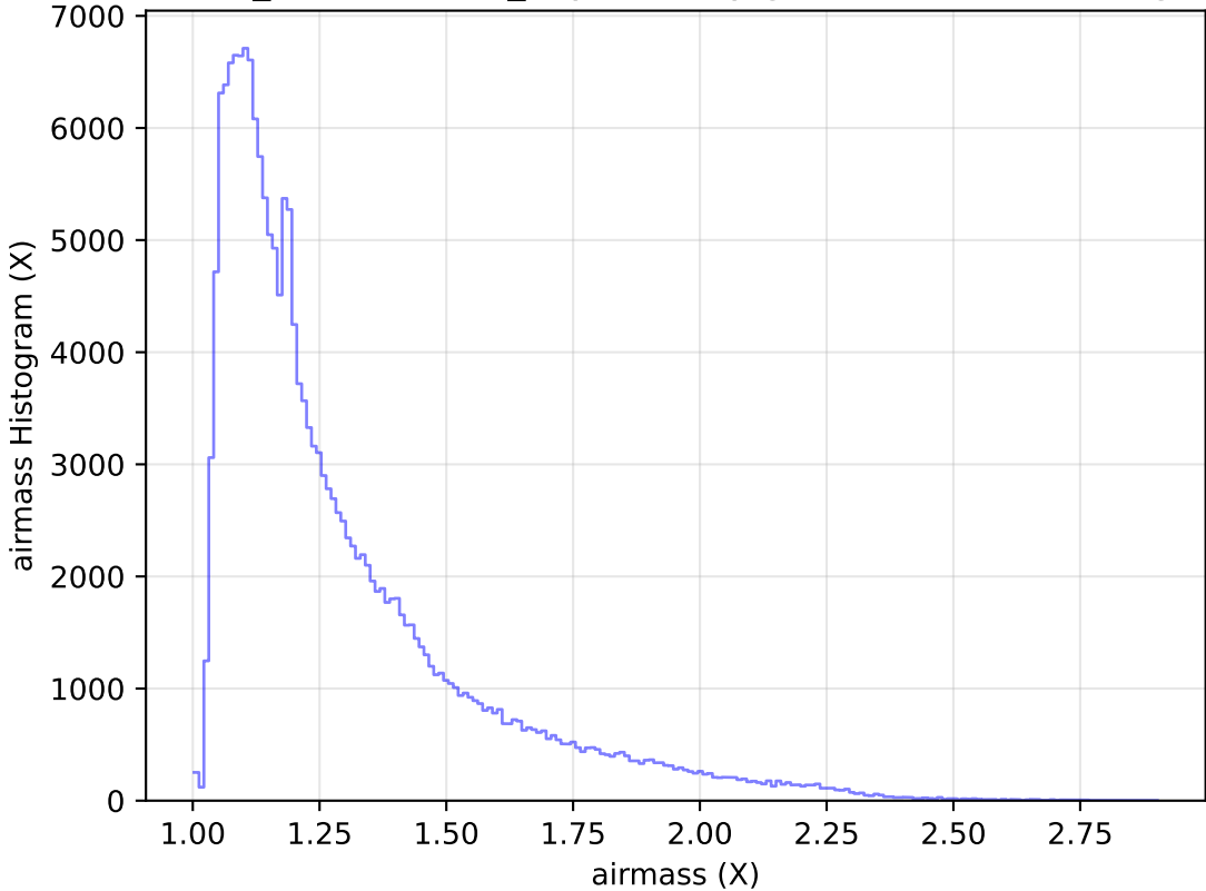
weather_cloudso2v3.4_10yrs All sky g band: airmass Histogram
