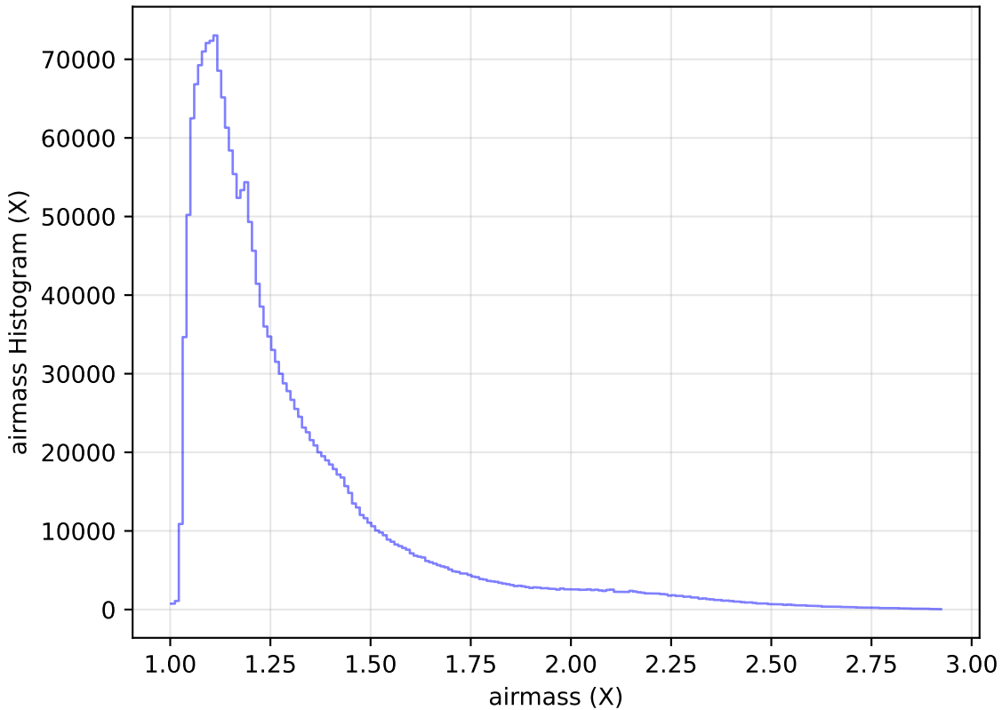
weather_cloudso2v3.4_10yrs All sky all bands: airmass Histogram
