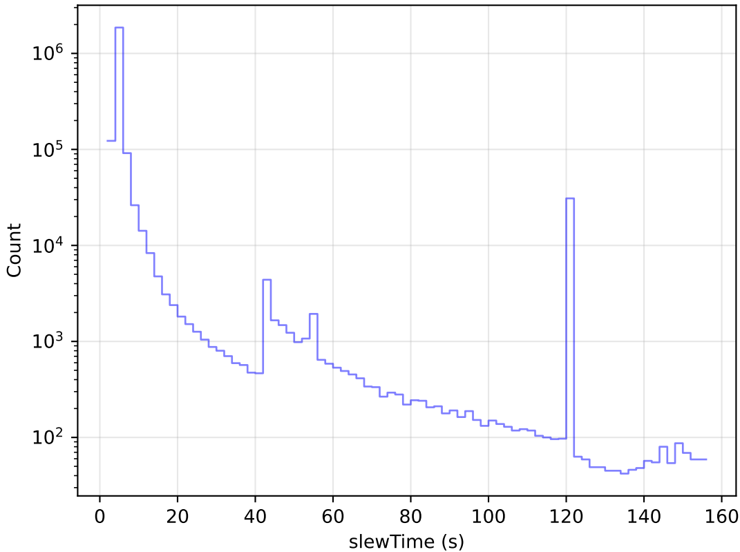
weather_cloudso2v3.4_10yrs All visits: Slew Time Histogram
