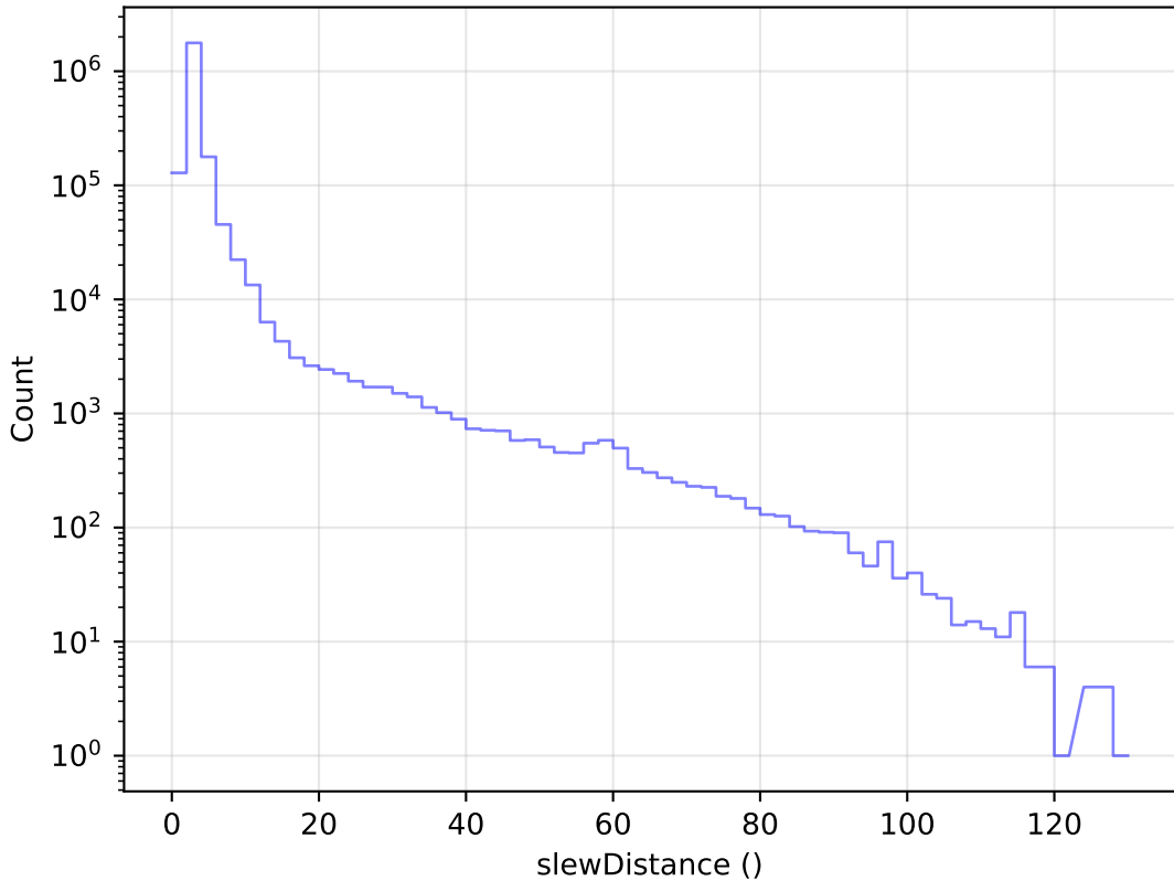
weather_cloudso2v3.4_10yrs All visits: Slew Distance Histogram
