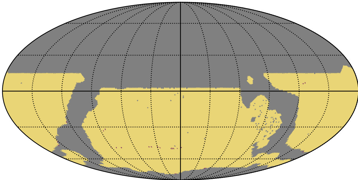
weather_cloudso2v3.4_10yrs WFD: RapidRevisits
