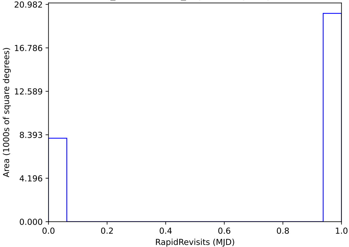
weather_cloudso2v3.4_10yrs All sky: RapidRevisits
