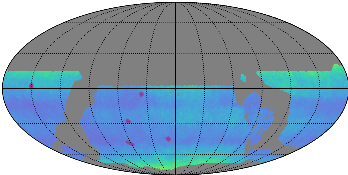
weather_cloudso2v3.4_10yrs WFD: Proper Motion Uncert @ 24.0
