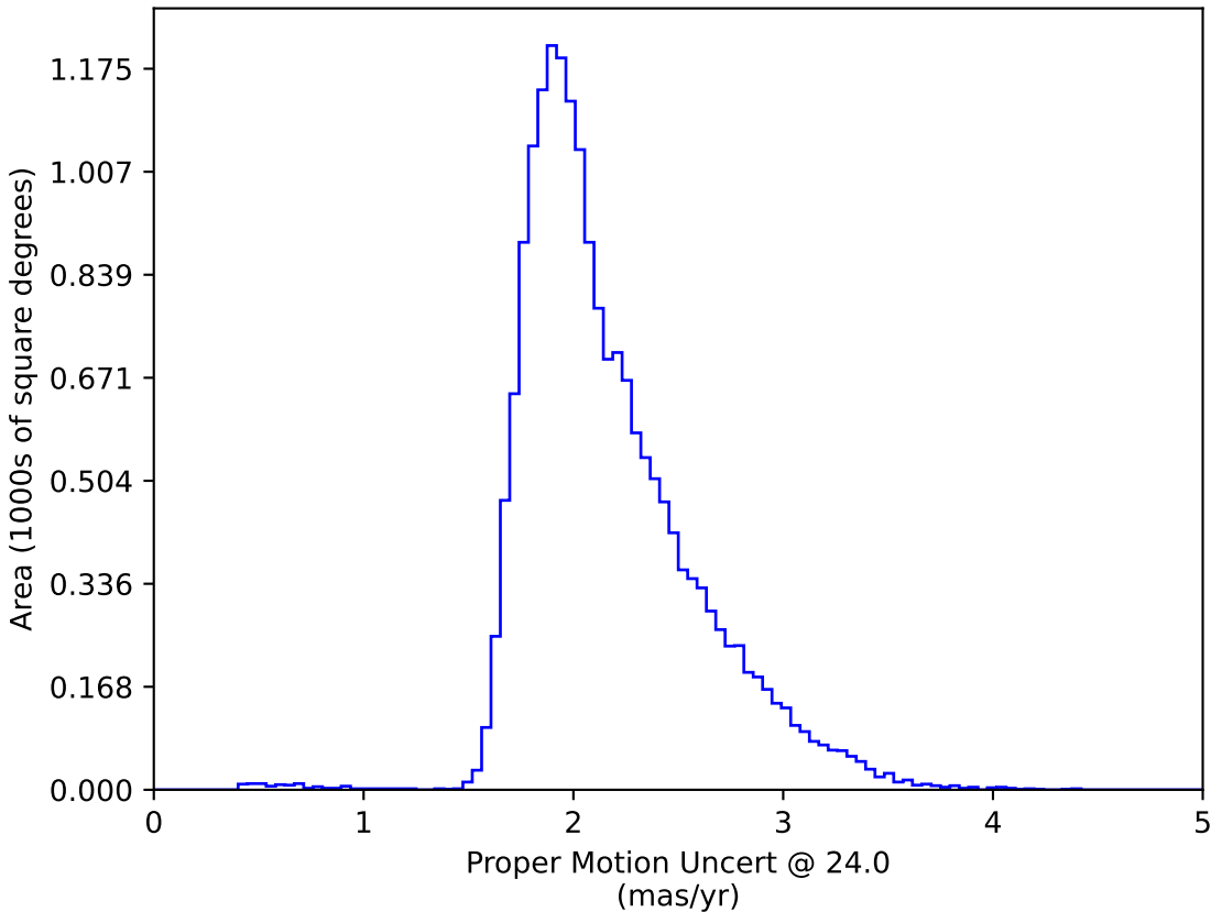
weather_cloudso2v3.4_10yrs WFD: Proper Motion Uncert @ 24.0
