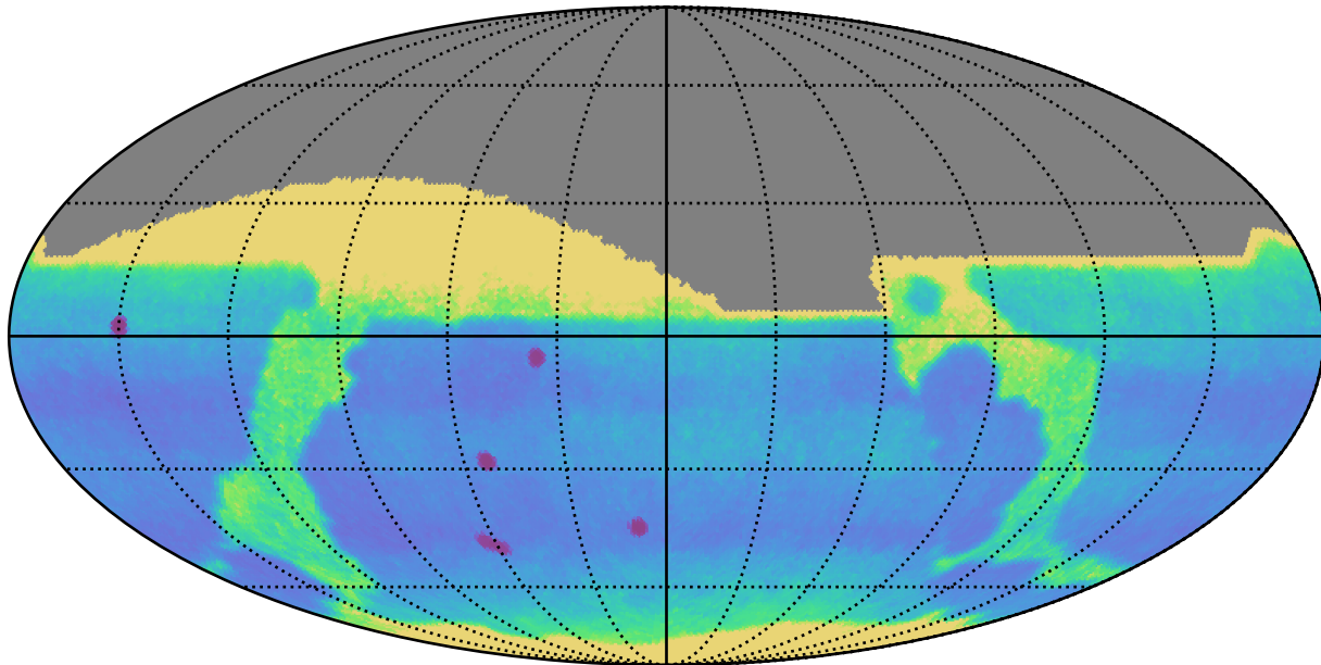
weather_cloudso2v3.4_10yrs All sky: Proper Motion Uncert @ 24.0
