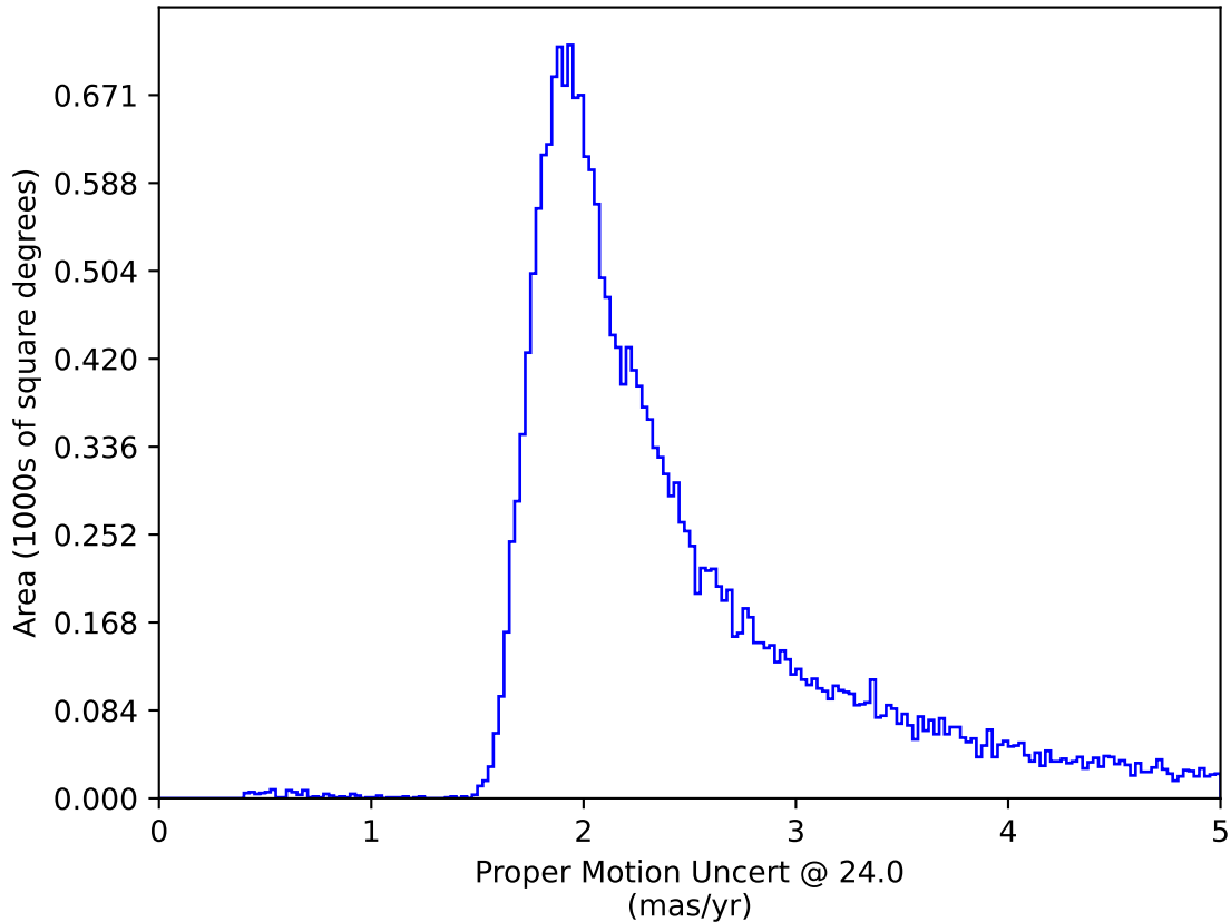
weather_cloudso2v3.4_10yrs All sky: Proper Motion Uncert @ 24.0
