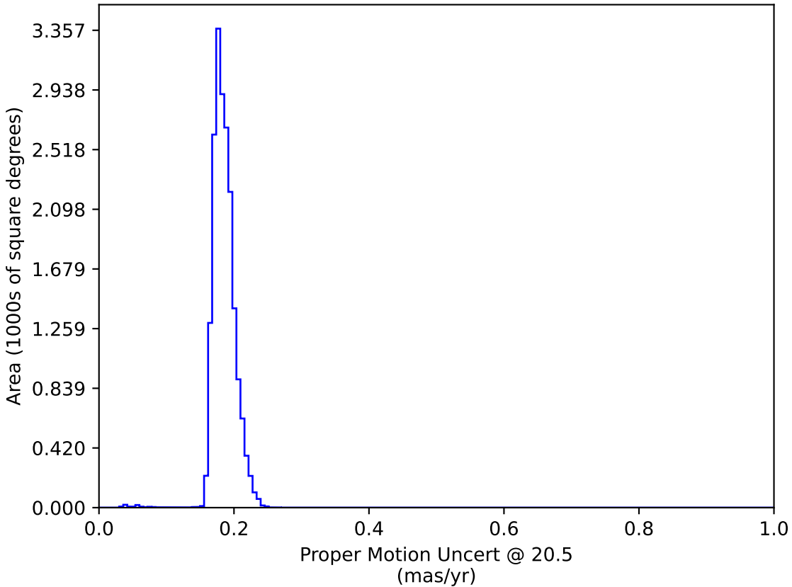
weather_cloudso2v3.4_10yrs WFD: Proper Motion Uncert @ 20.5
