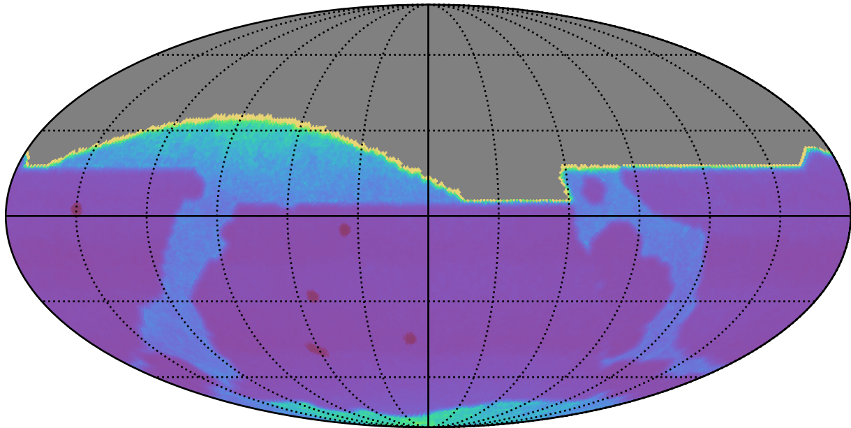
weather_cloudso2v3.4_10yrs All sky: Proper Motion Uncert @ 20.5
