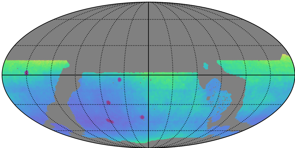
weather_cloudso2v3.4_10yrs WFD: Parallax Uncert @ 24.0
