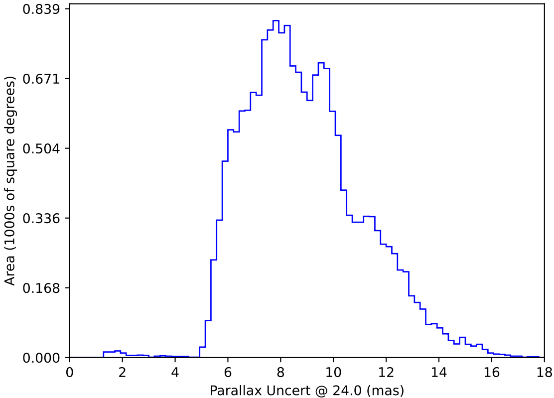
weather_cloudso2v3.4_10yrs WFD: Parallax Uncert @ 24.0
