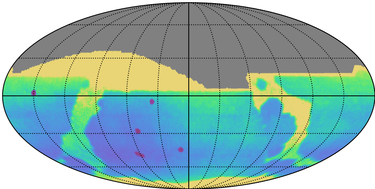
weather_cloudso2v3.4_10yrs All sky: Parallax Uncert @ 24.0
