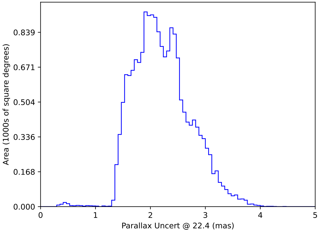
weather_cloudso2v3.4_10yrs WFD: Parallax Uncert @ 22.4
