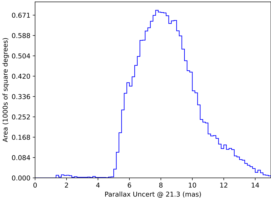
weather_cloudso2v3.4_10yrs WFD y band only: Parallax Uncert @ 21.3
