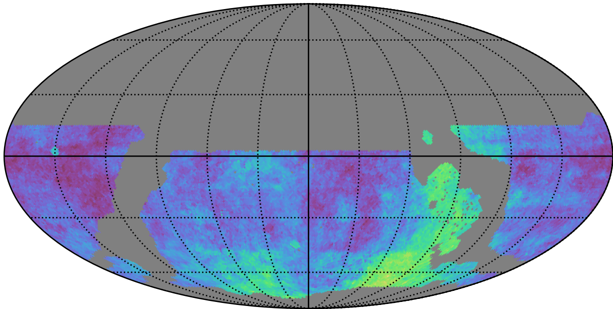
weather_cloudso2v3.4_10yrs WFD: Parallax Coverage @ 24.0
