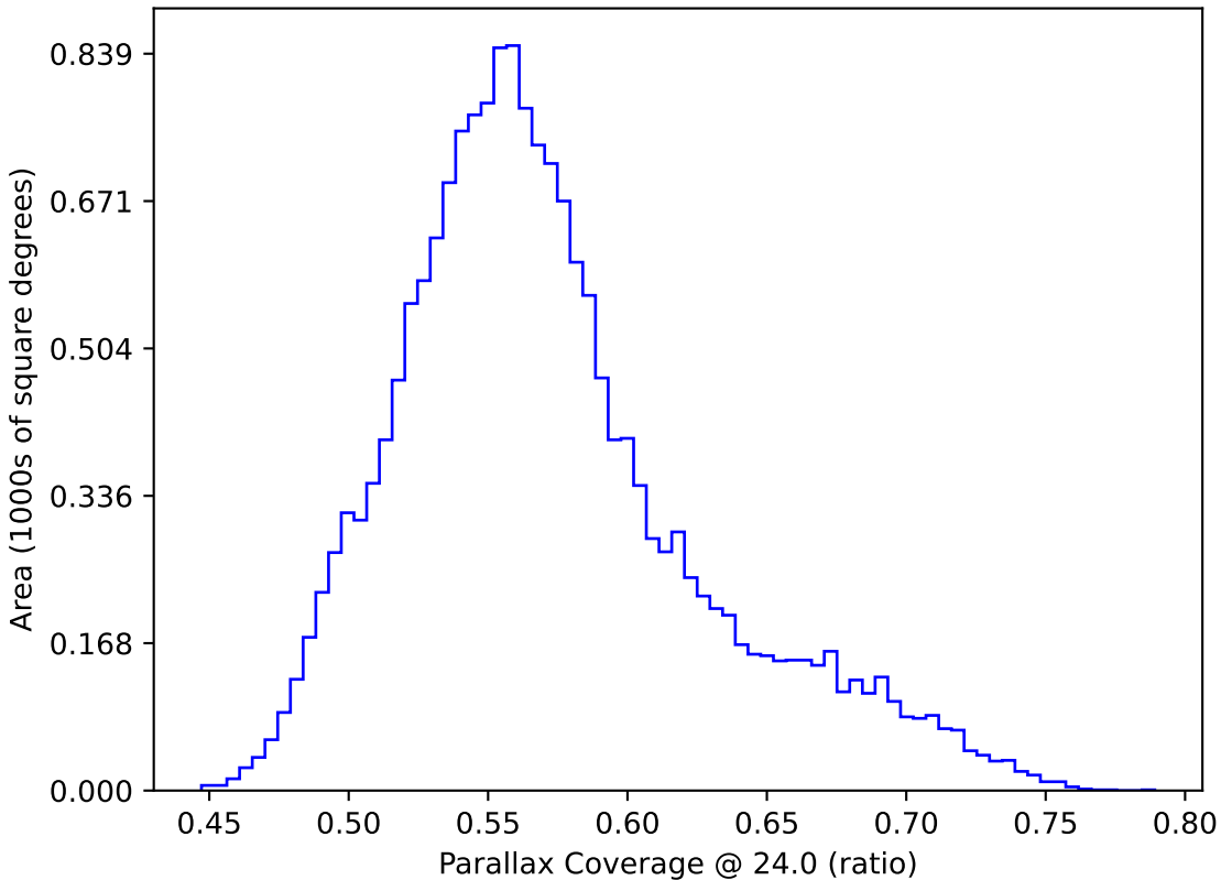
weather_cloudso2v3.4_10yrs WFD: Parallax Coverage @ 24.0
