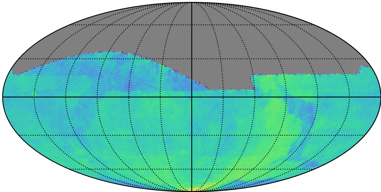
weather_cloudso2v3.4_10yrs All sky: Parallax Coverage @ 24.0
