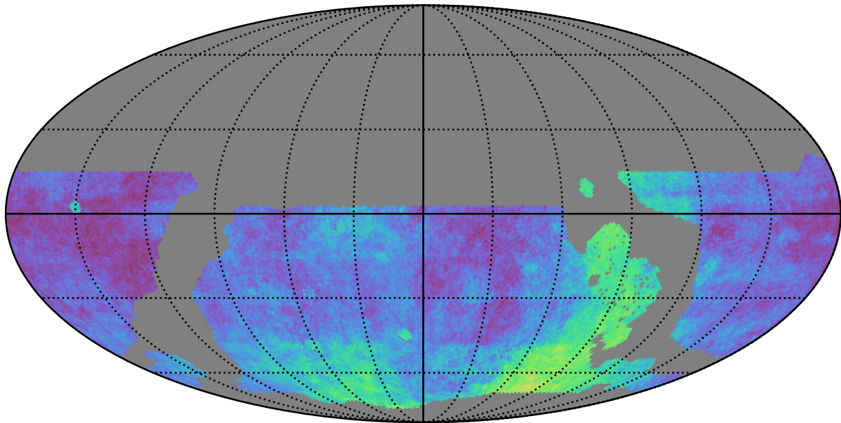
weather_cloudso2v3.4_10yrs WFD: Parallax Coverage @ 22.4
