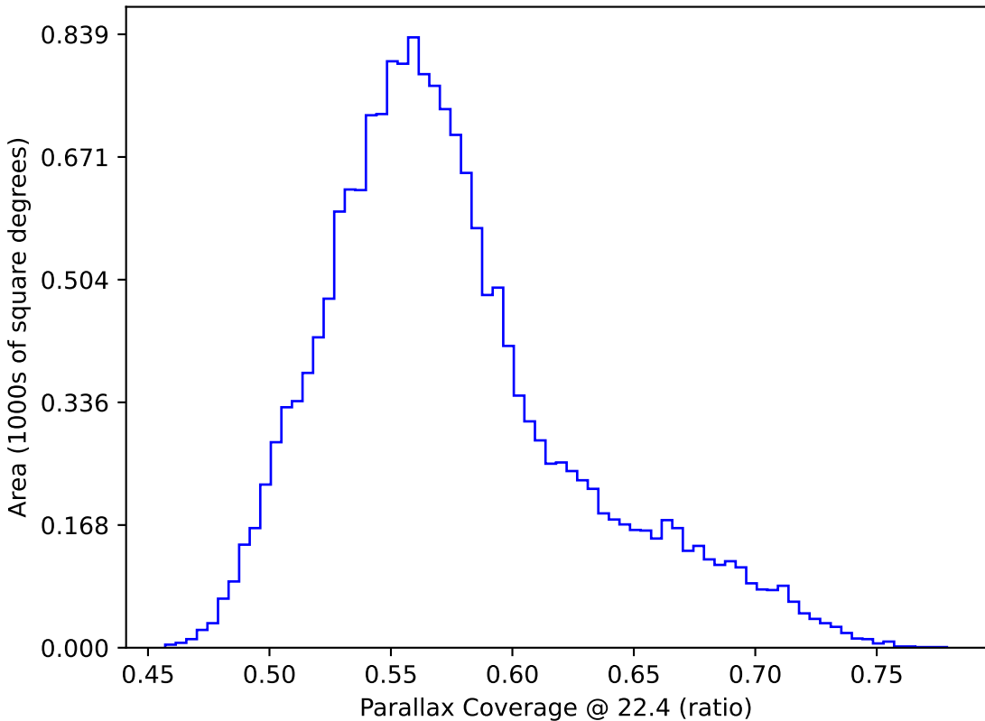
weather_cloudso2v3.4_10yrs WFD: Parallax Coverage @ 22.4
