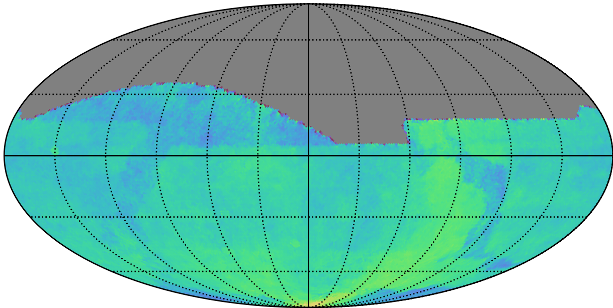
weather_cloudso2v3.4_10yrs All sky: Parallax Coverage @ 22.4
