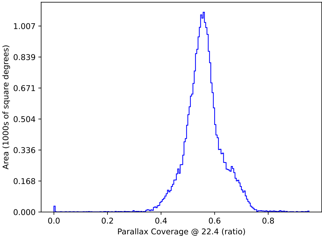
weather_cloudso2v3.4_10yrs All sky: Parallax Coverage @ 22.4
