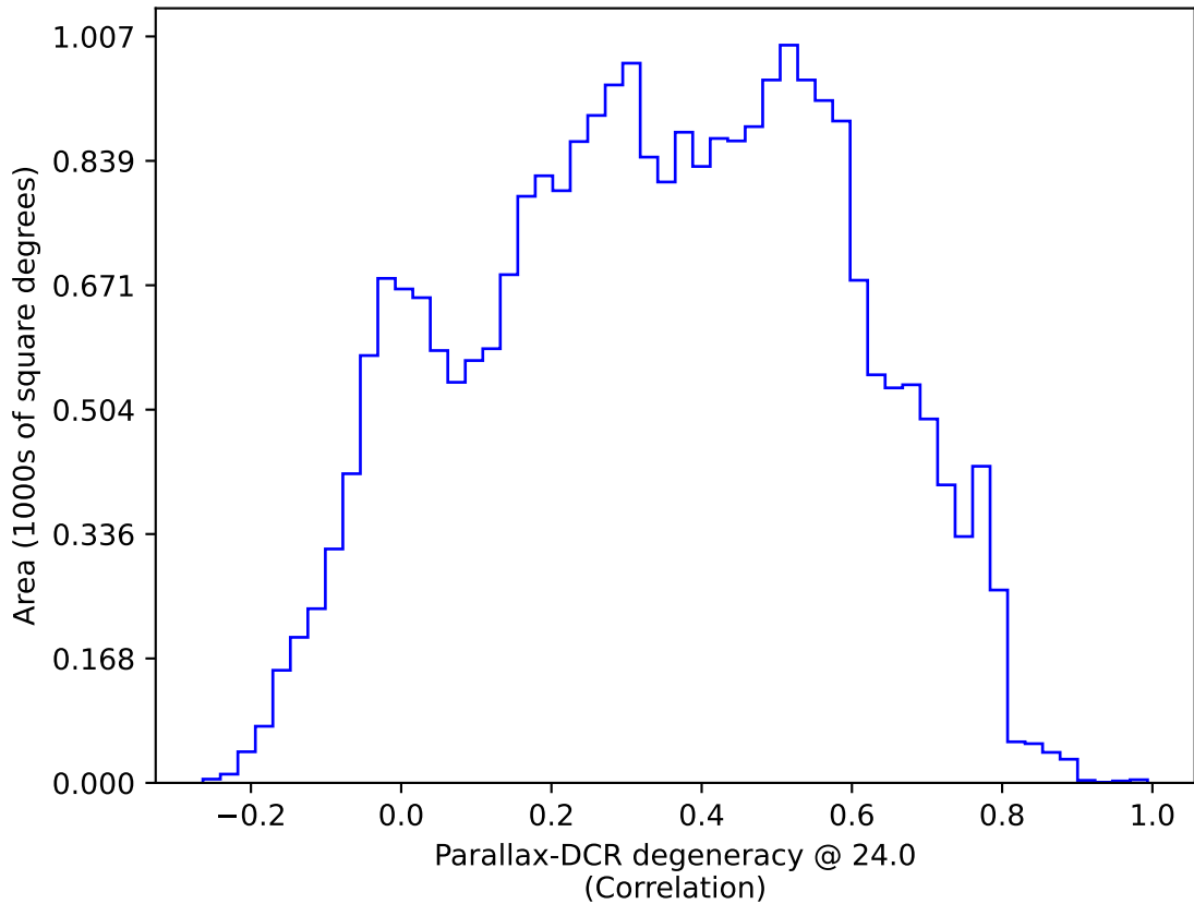
weather_cloudso2v3.4_10yrs All sky: Parallax-DCR degeneracy @ 24.0
