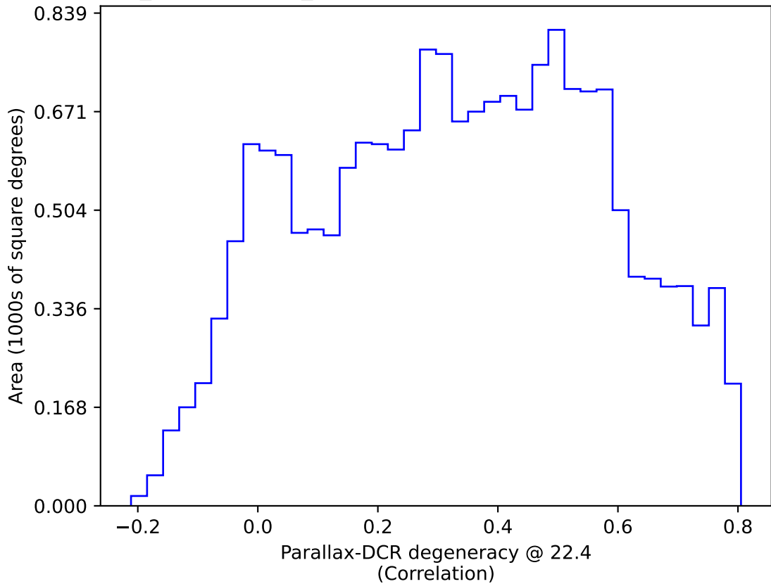
weather_cloudso2v3.4_10yrs WFD: Parallax-DCR degeneracy @ 22.4
