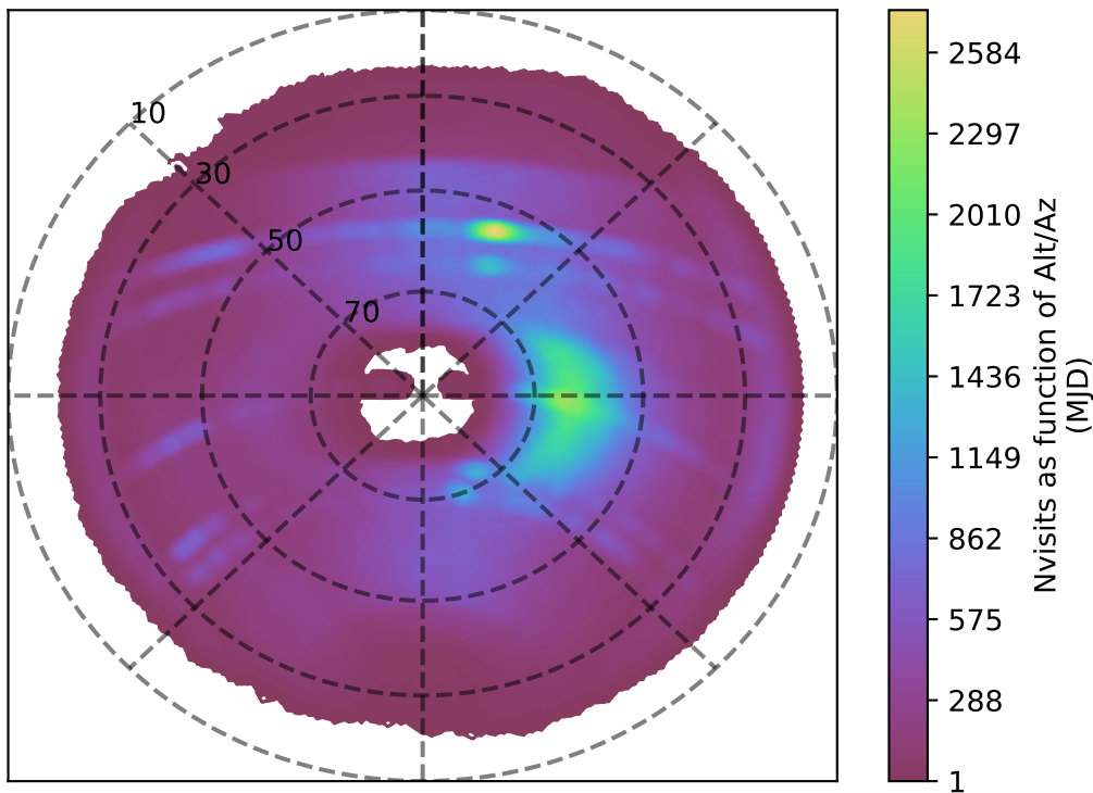
weather_cloudso2v3.4_10yrs z band: Nvisits as function of Alt/Az
