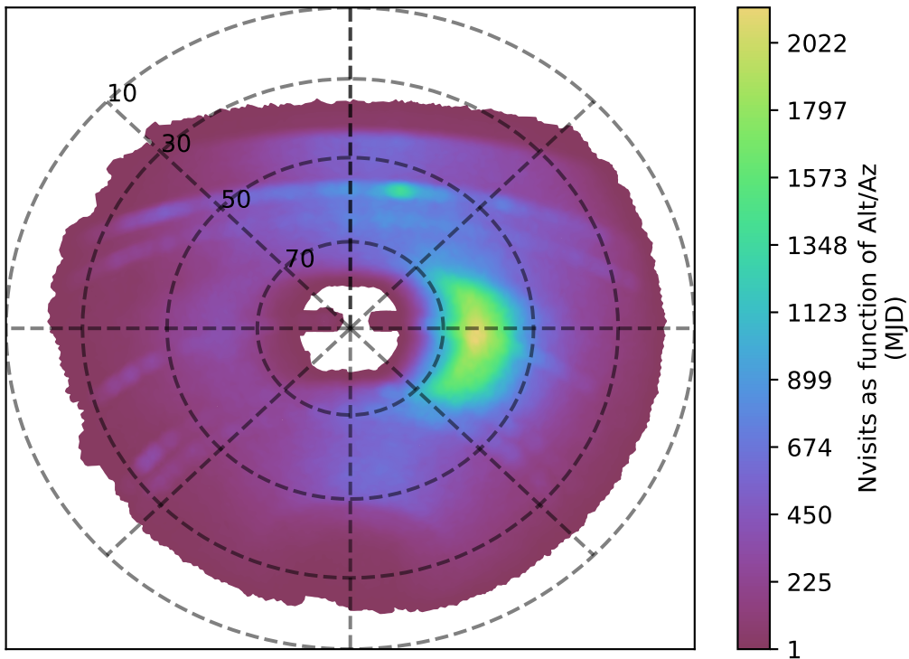
weather_cloudso2v3.4_10yrs y band: Nvisits as function of Alt/Az
