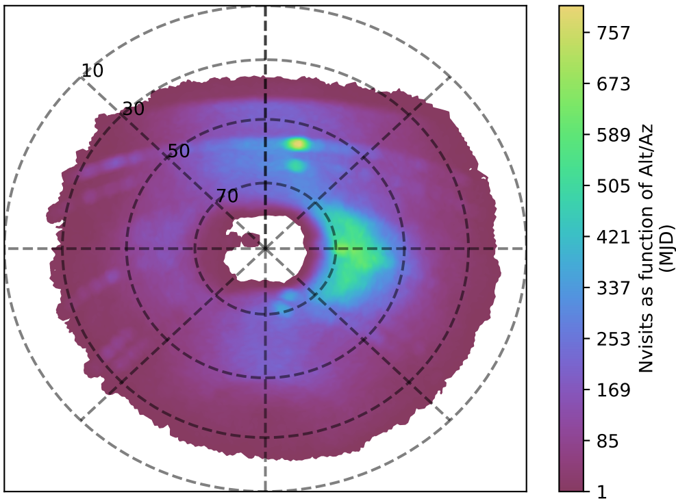
weather_cloudso2v3.4_10yrs u band: Nvisits as function of Alt/Az
