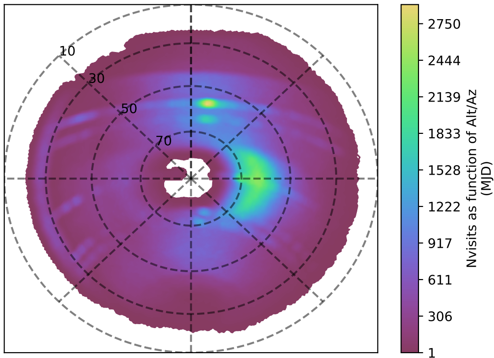
weather_cloudso2v3.4_10yrs r band: Nvisits as function of Alt/Az
